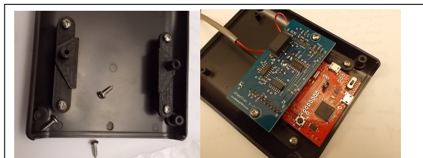
Figure 2. Standoffs are attached loosely to the bottom of the case with angled edges pointing inward. The boards are slid into place with the red board held under the angled edge. The amplifier board is held to the standoffs using 3/8" #4 sheet metal screws.
